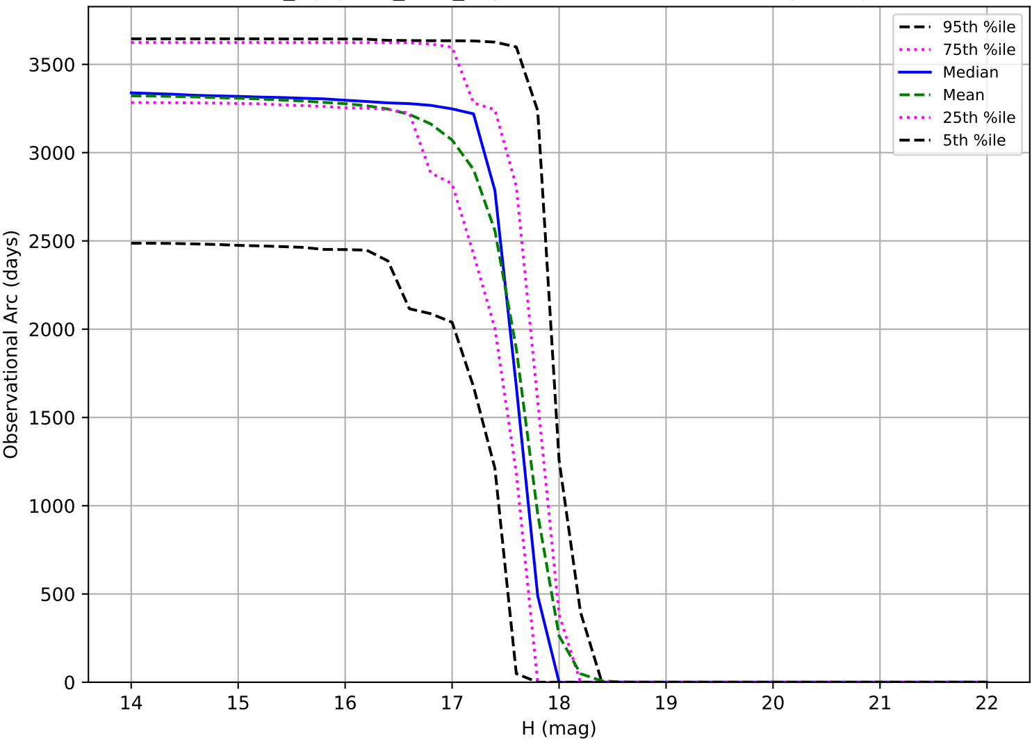
noroll_mjdp180_v3.4_10yrs: Observational Arc Length Trojan
