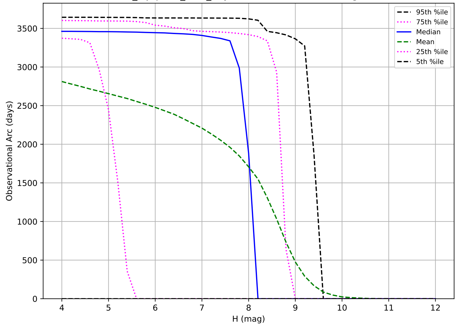
noroll_mjdp180_v3.4_10yrs: Observational Arc Length TNO
