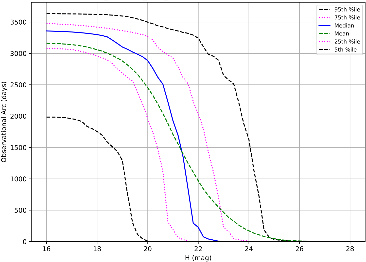
noroll_mjdp180_v3.4_10yrs: Observational Arc Length PHA
