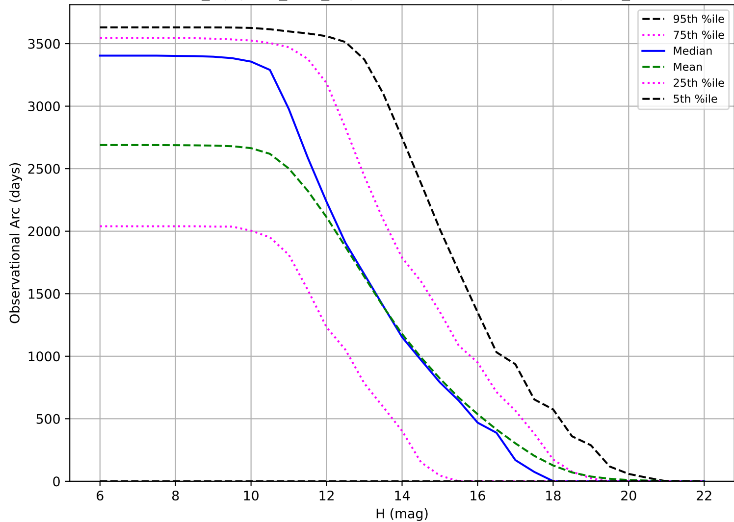
noroll_mjdp180_v3.4_10yrs: Observational Arc Length OCC_r5
