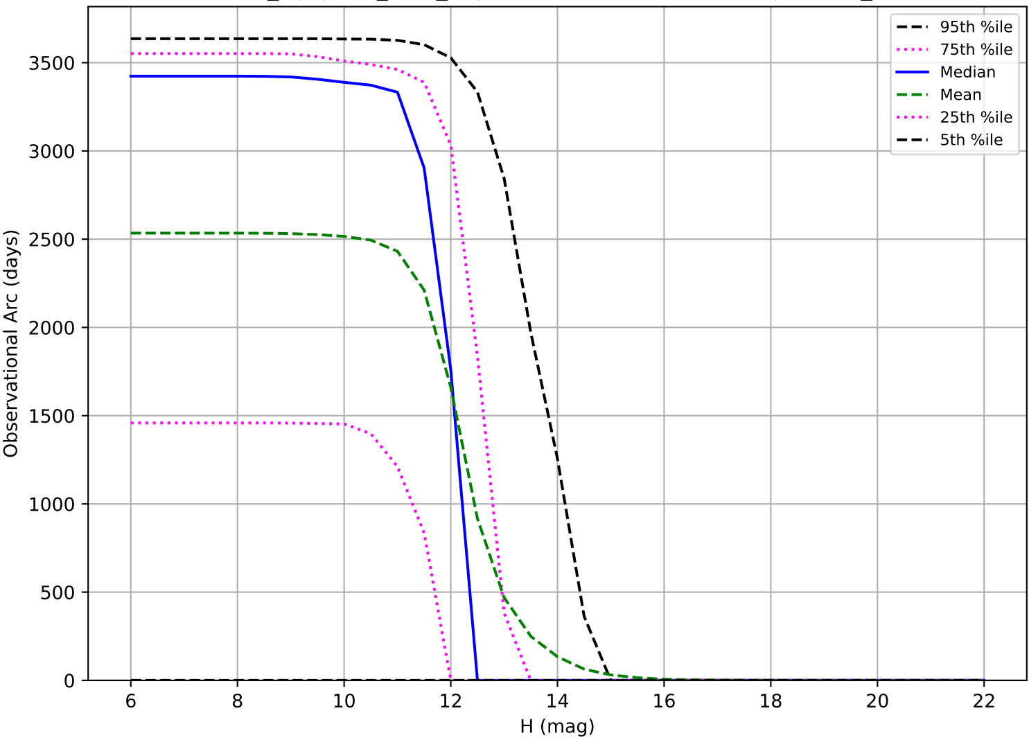
noroll_mjdp180_v3.4_10yrs: Observational Arc Length OCC_r20
