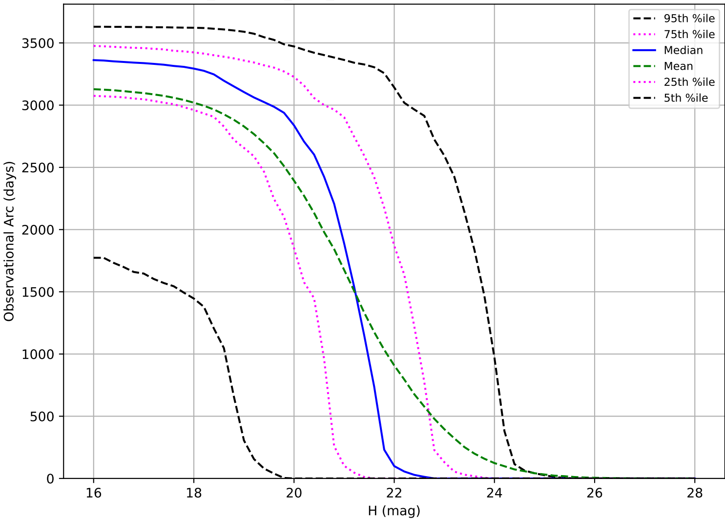
noroll_mjdp180_v3.4_10yrs: Observational Arc Length NEO
