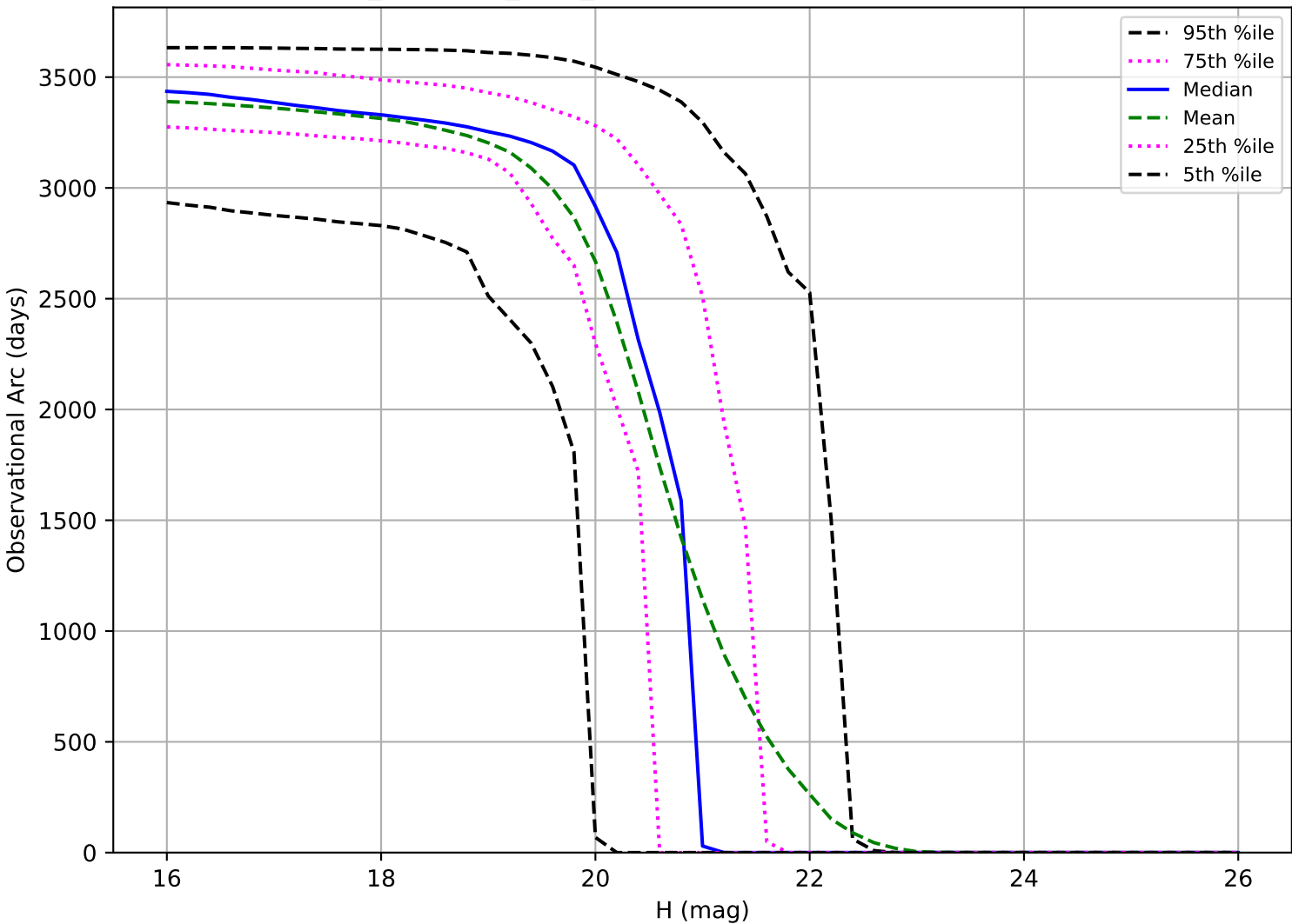
noroll_mjdp180_v3.4_10yrs: Observational Arc Length MBA
