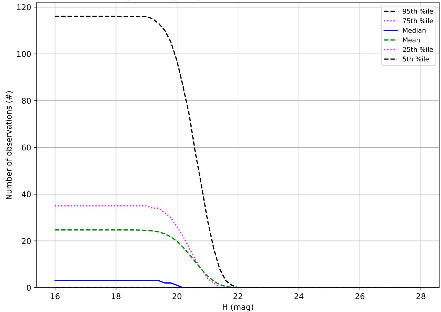
noroll_mjdp180_v3.4_10yrs: Number of observations Vatira
