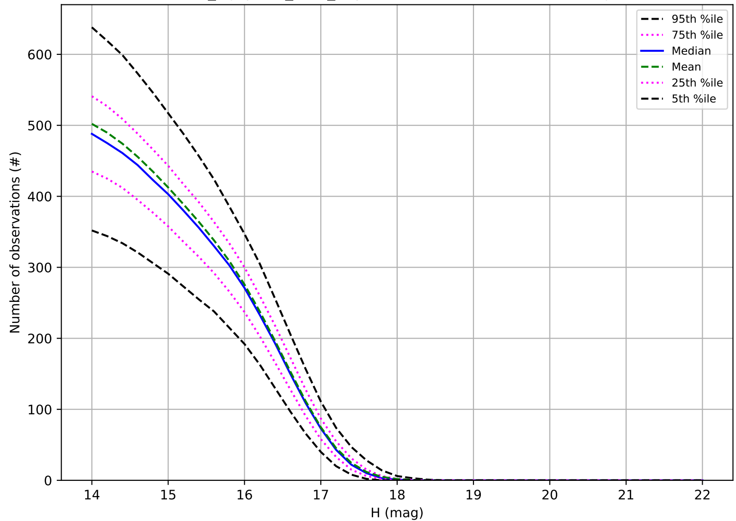
noroll_mjdp180_v3.4_10yrs: Number of observations Trojan
