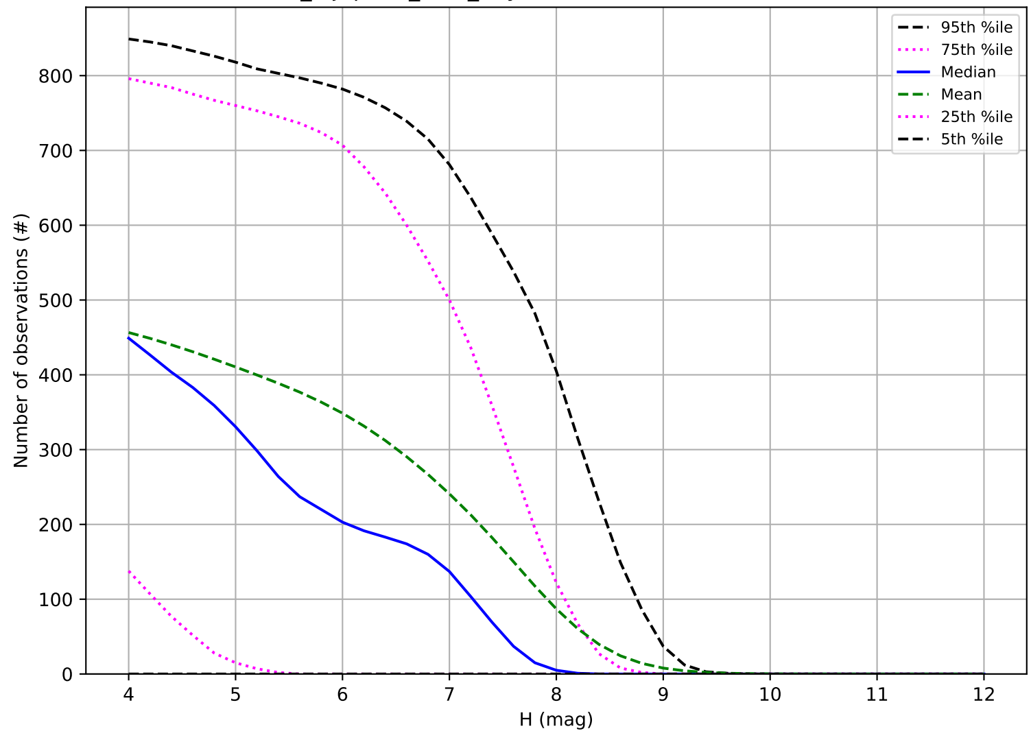
noroll_mjdp180_v3.4_10yrs: Number of observations TNO
