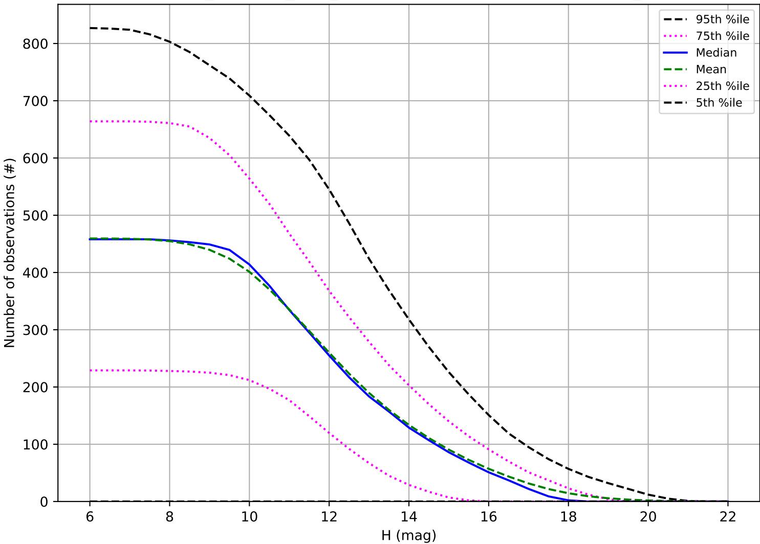
noroll_mjdp180_v3.4_10yrs: Number of observations OCC_r5
