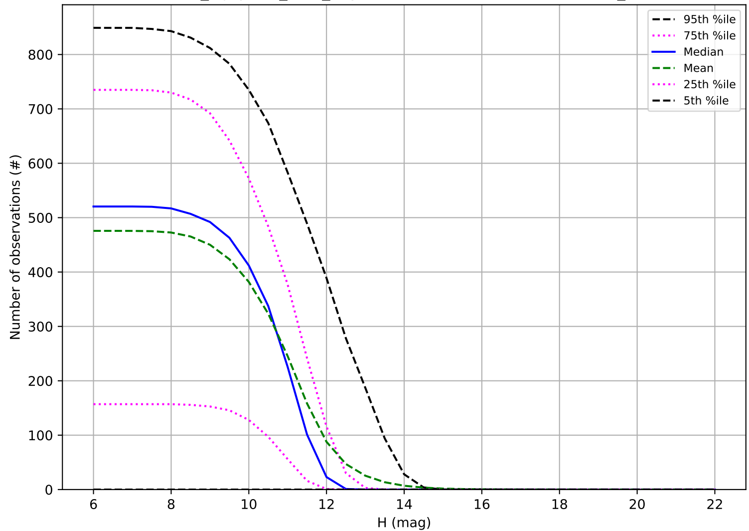
noroll_mjdp180_v3.4_10yrs: Number of observations OCC_r20
