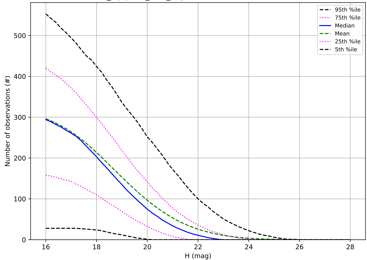
noroll_mjdp180_v3.4_10yrs: Number of observations NEO
