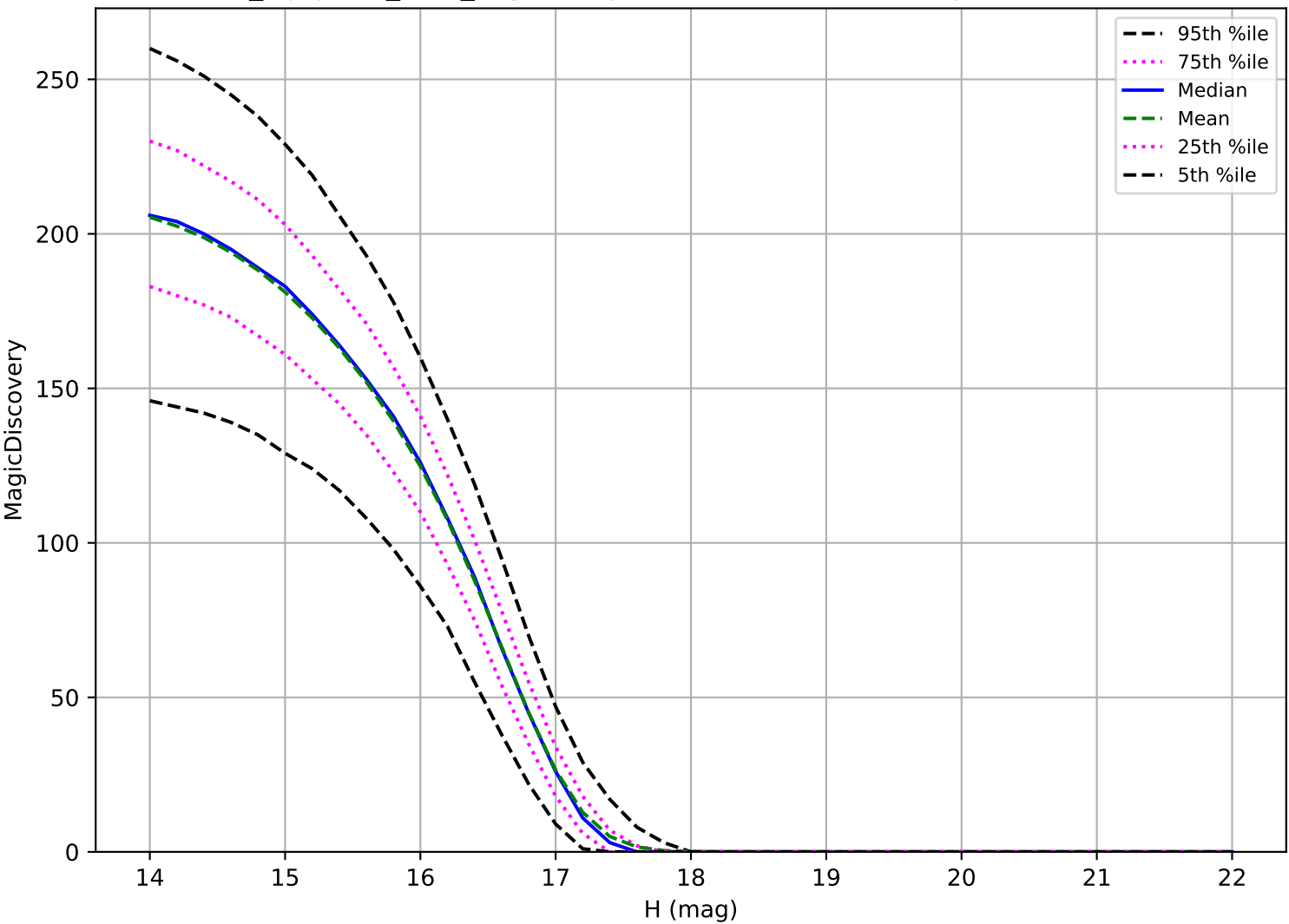
noroll_mjdp180_v3.4_10yrs: Trojan 6 detections in 60 nights detection loss
