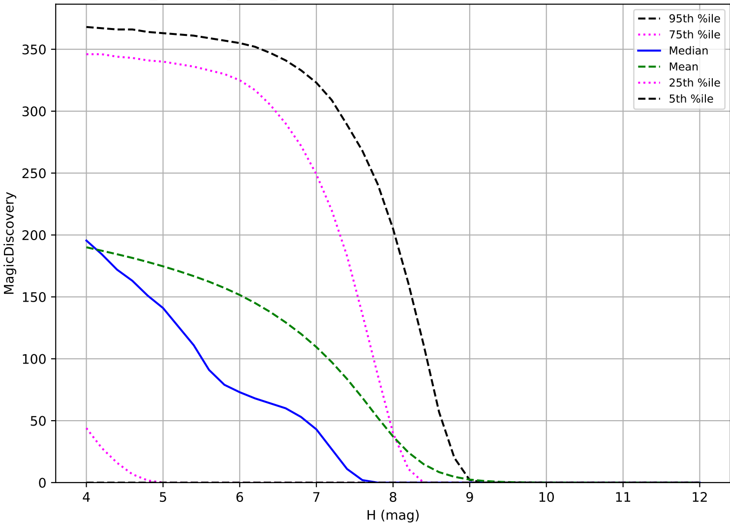
noroll_mjdp180_v3.4_10yrs: TNO 6 detections in 60 nights detection loss
