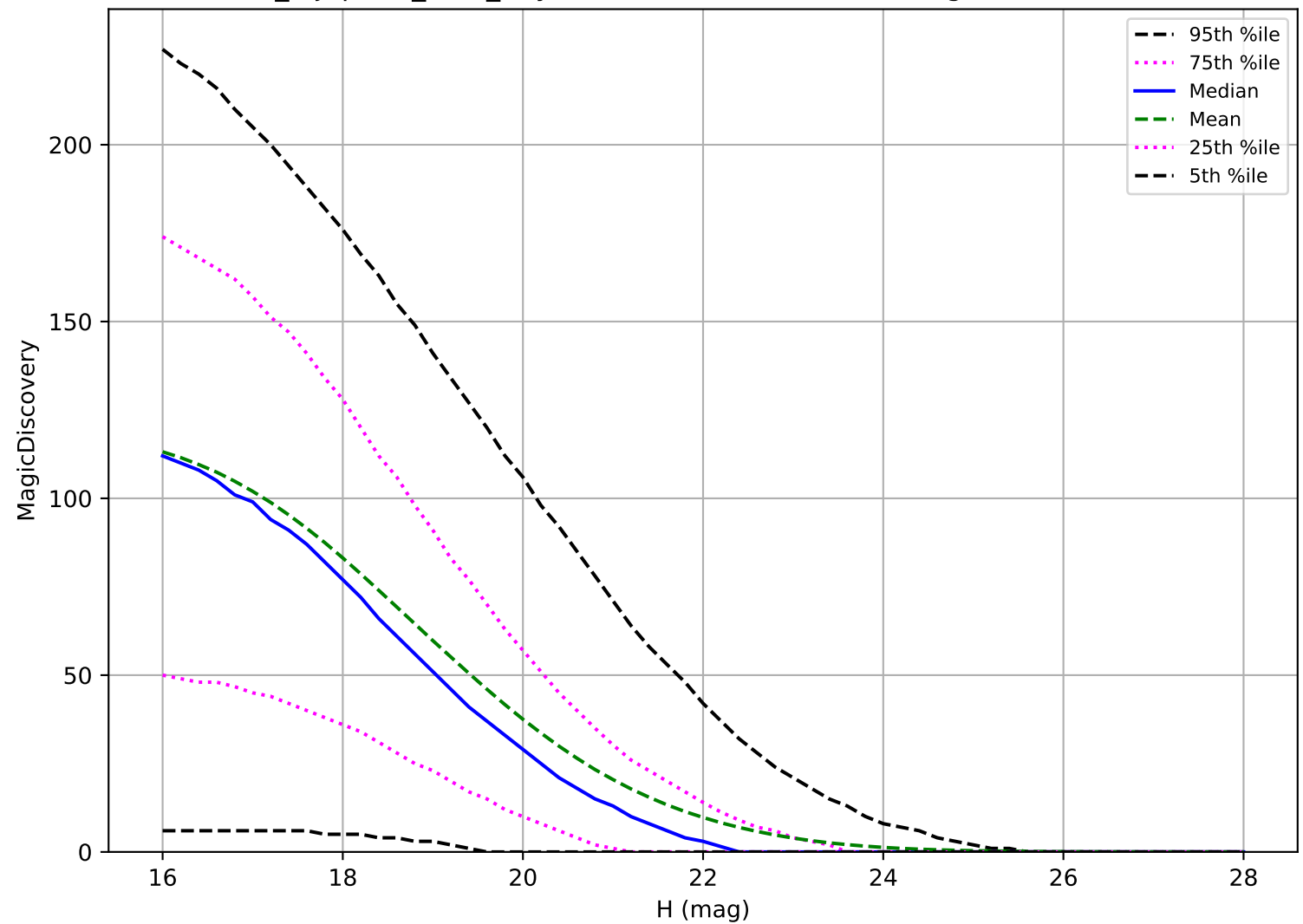
noroll_mjdp180_v3.4_10yrs: PHA 6 detections in 60 nights detection loss
