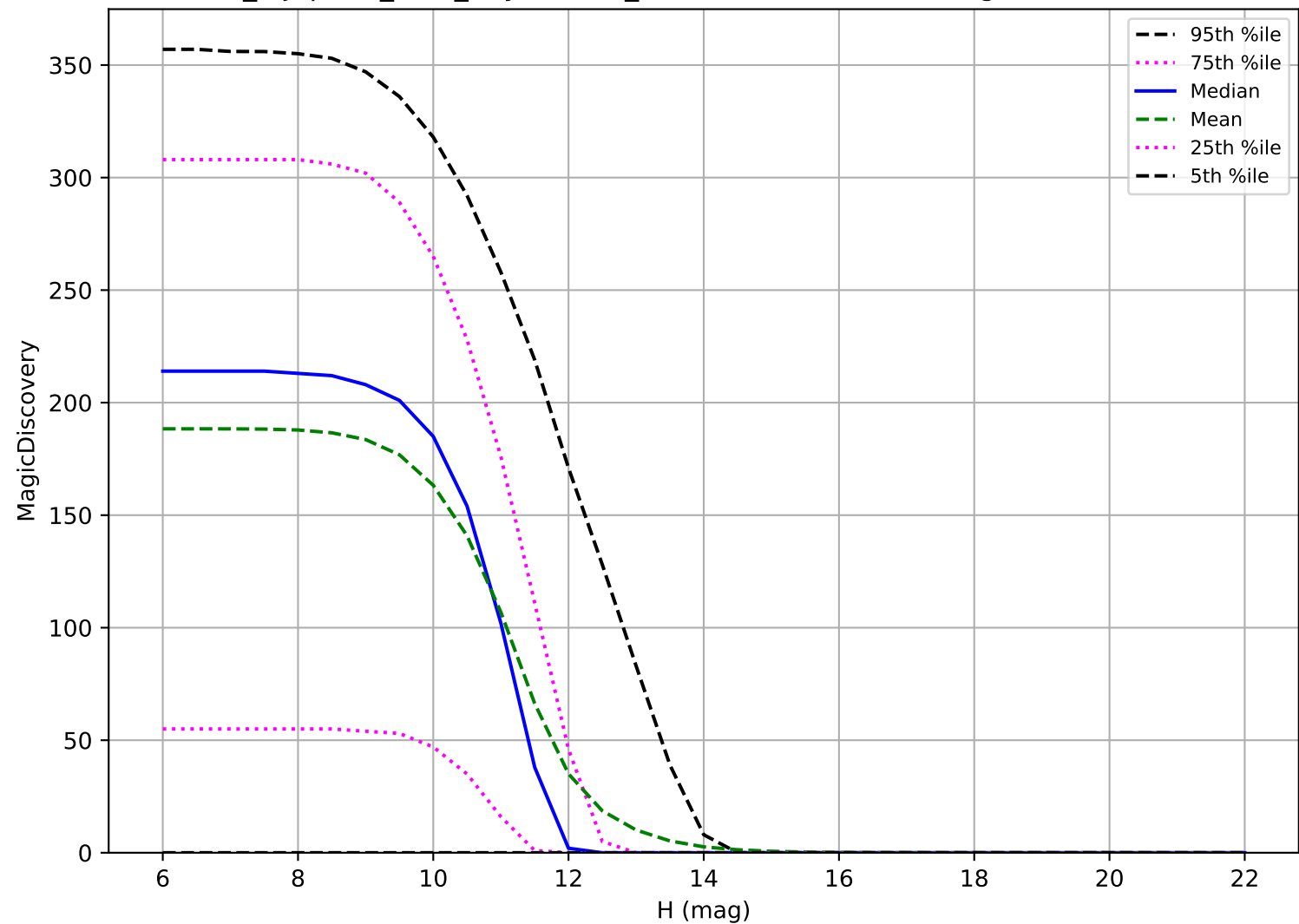
noroll_mjdp180_v3.4_10yrs: OCC_r20 6 detections in 60 nights detection loss
