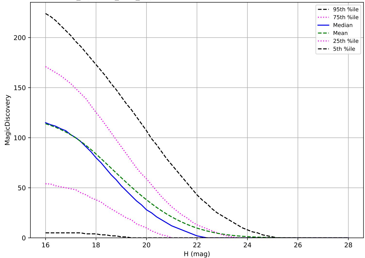
noroll_mjdp180_v3.4_10yrs: NEO 6 detections in 60 nights detection loss
