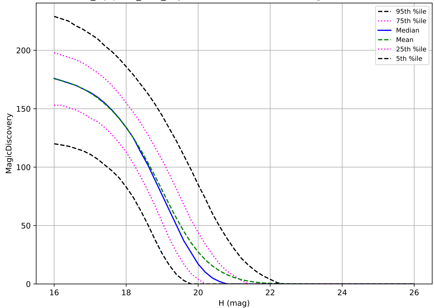
noroll_mjdp180_v3.4_10yrs: MBA 6 detections in 60 nights detection loss
