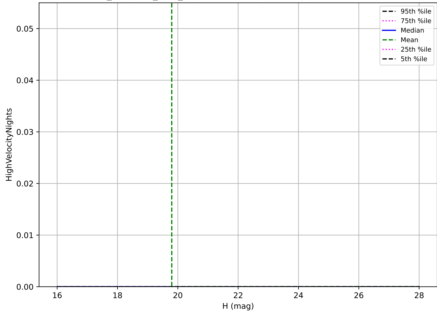
noroll_mjdp180_v3.4_10yrs: Vatira High velocity pair detection loss
