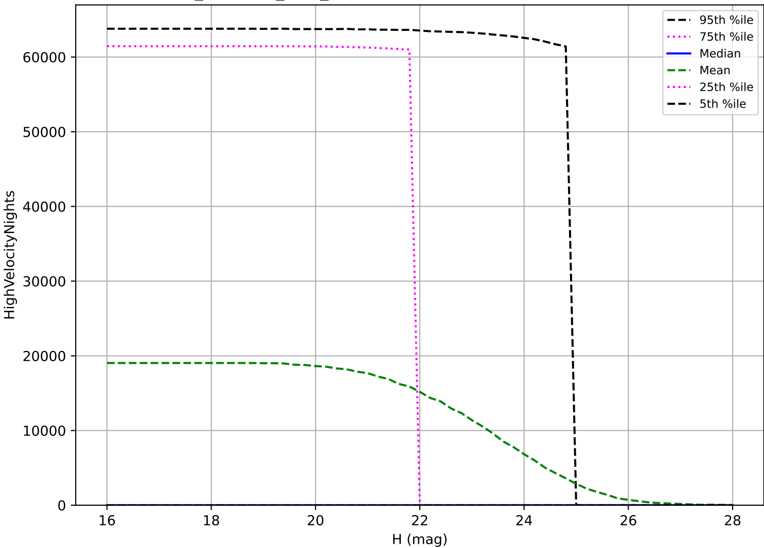
noroll_mjdp180_v3.4_10yrs: NEO High velocity pair detection loss
