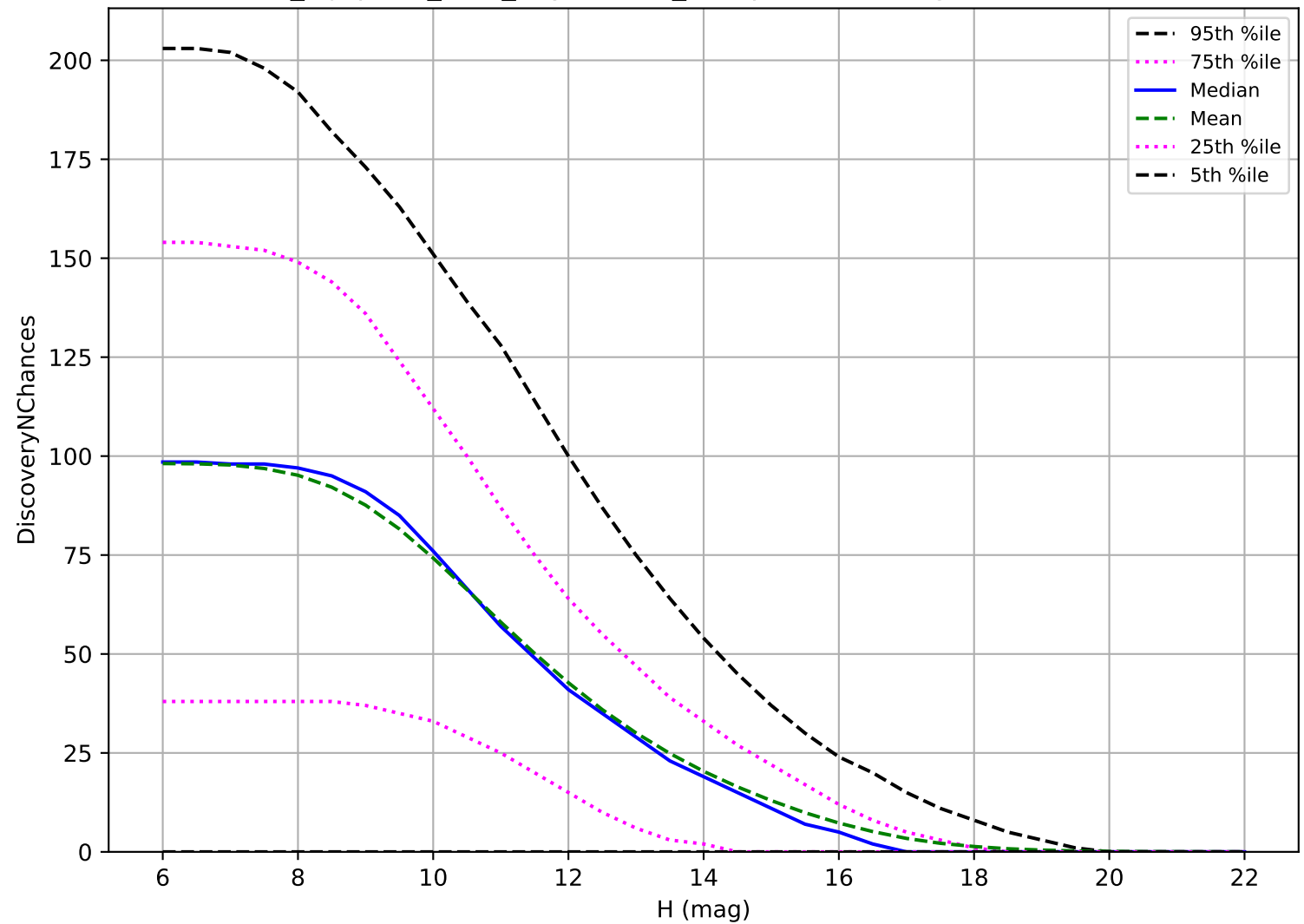
noroll_mjdp180_v3.4_10yrs: OCC_r5 3 pairs in 15 nights detection loss
