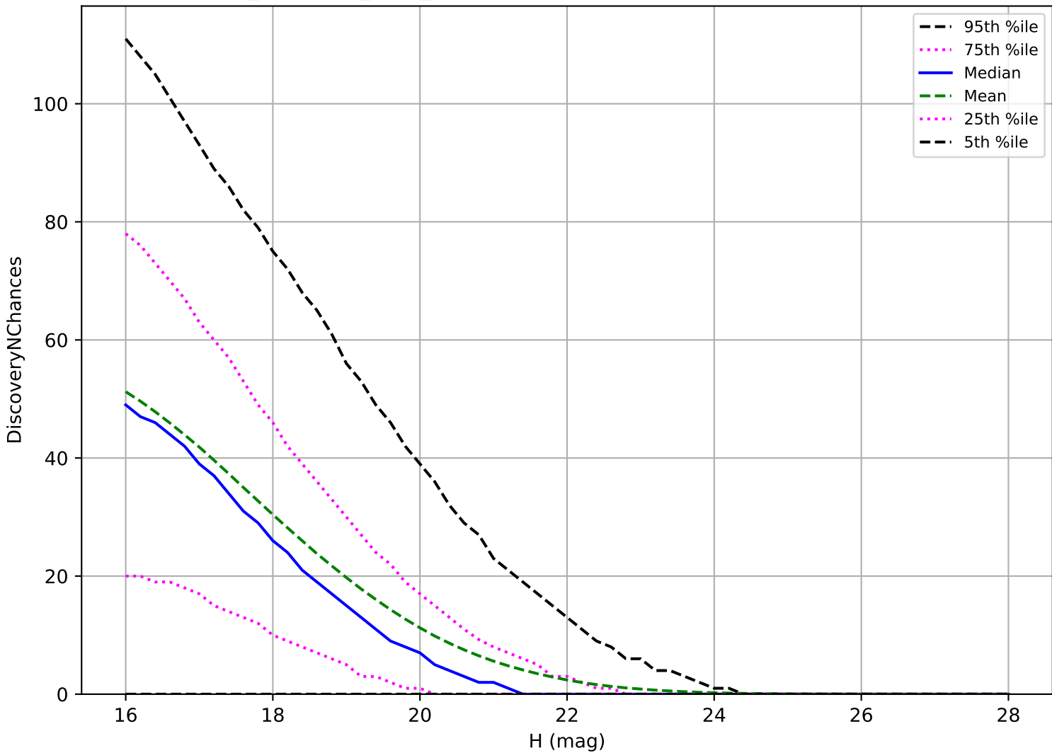
noroll_mjdp180_v3.4_10yrs: NEO 3 pairs in 15 nights detection loss
