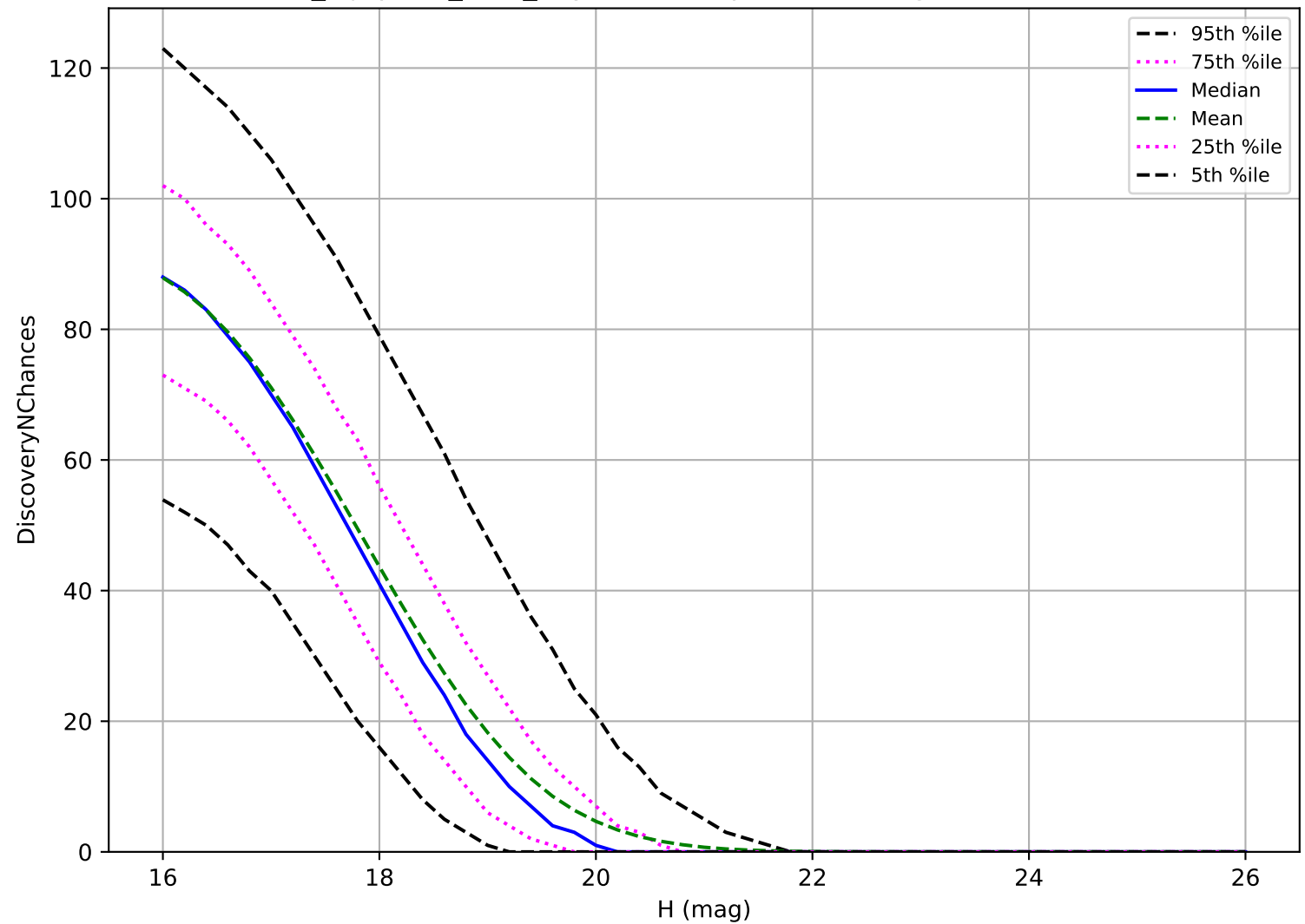
noroll_mjdp180_v3.4_10yrs: MBA 3 pairs in 15 nights detection loss
