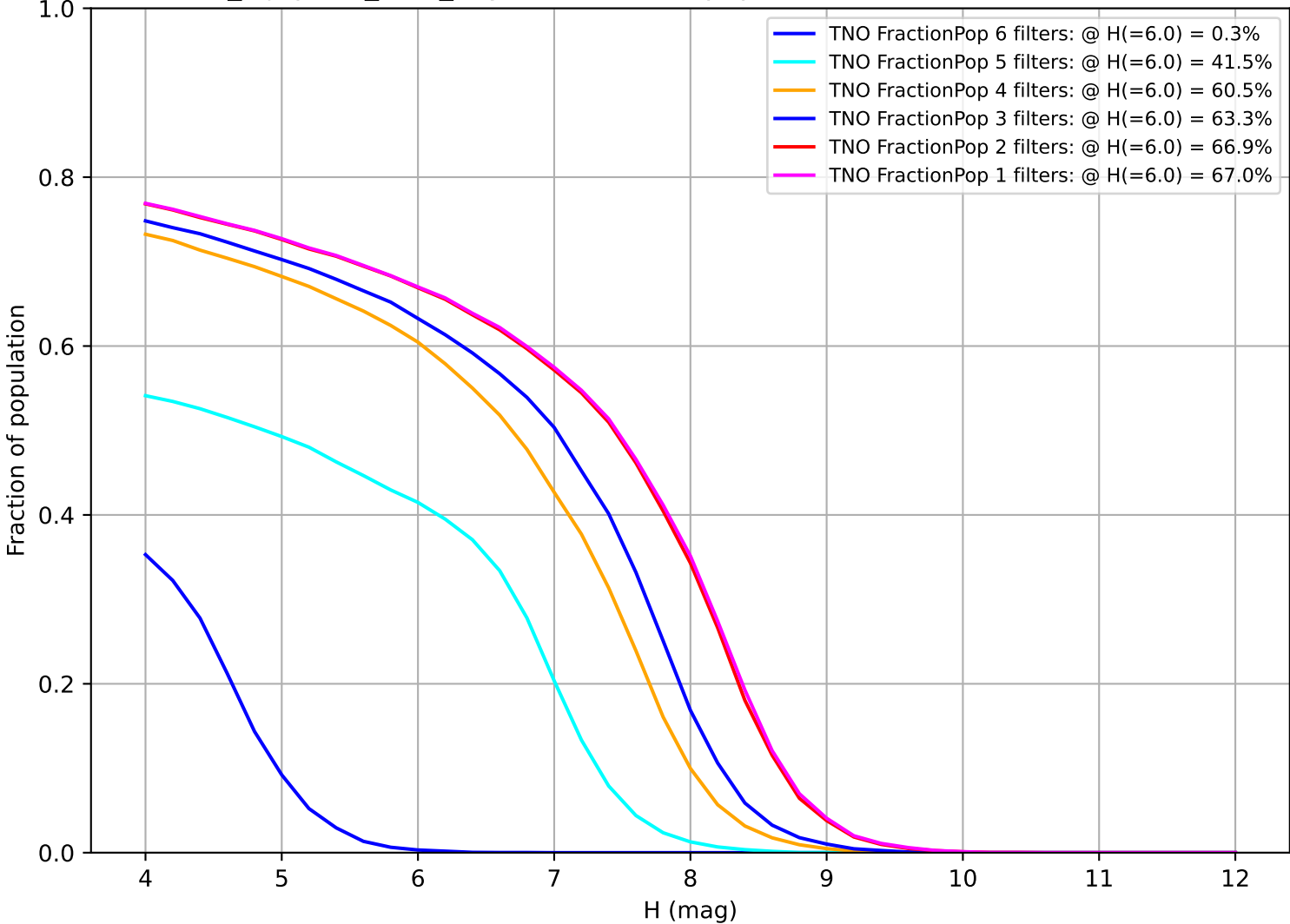
noroll_mjdp180_v3.4_10yrs: Fraction of population with colors in X filters TNO
