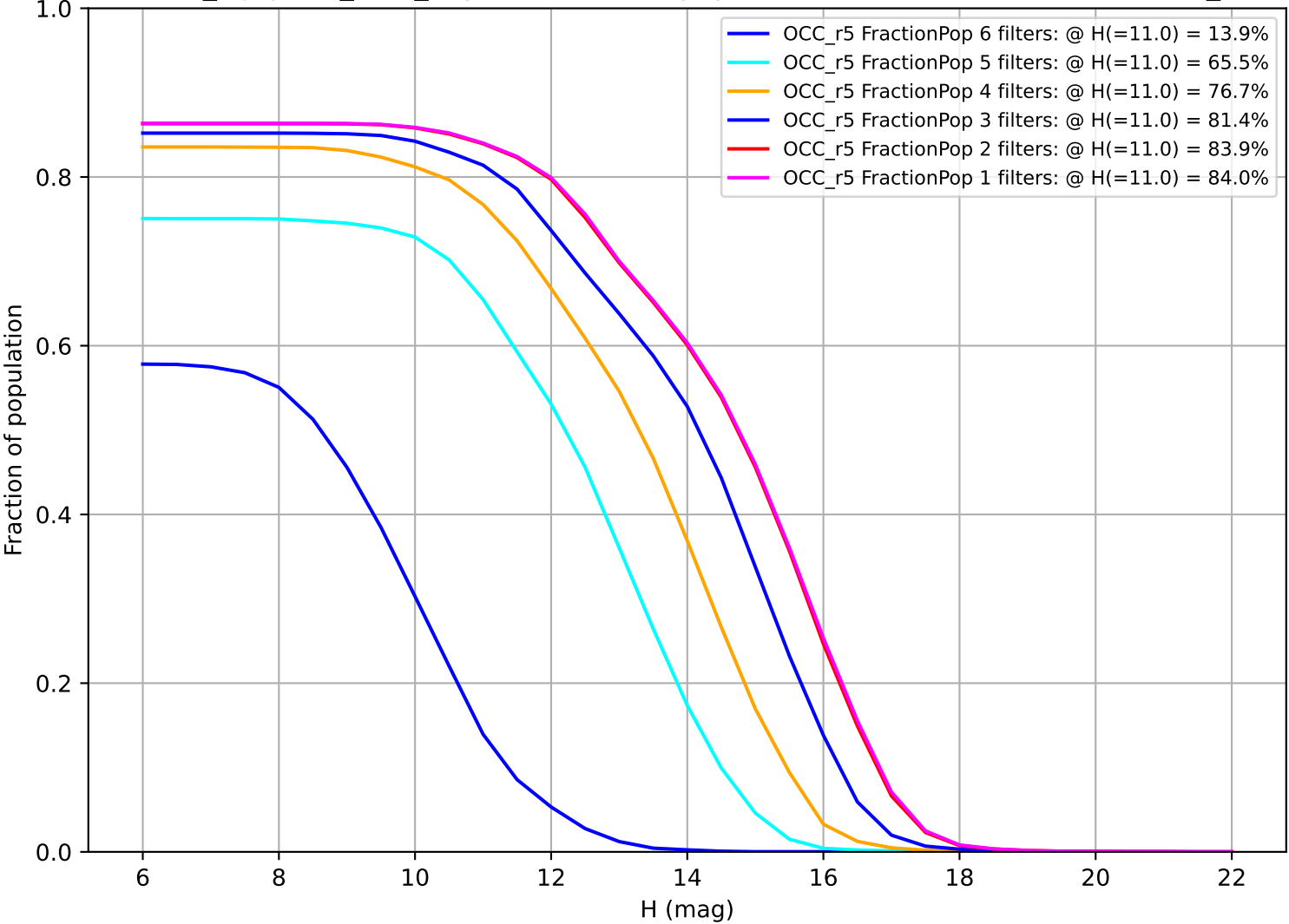
noroll_mjdp180_v3.4_10yrs: Fraction of population with colors in X filters OCC_r5
