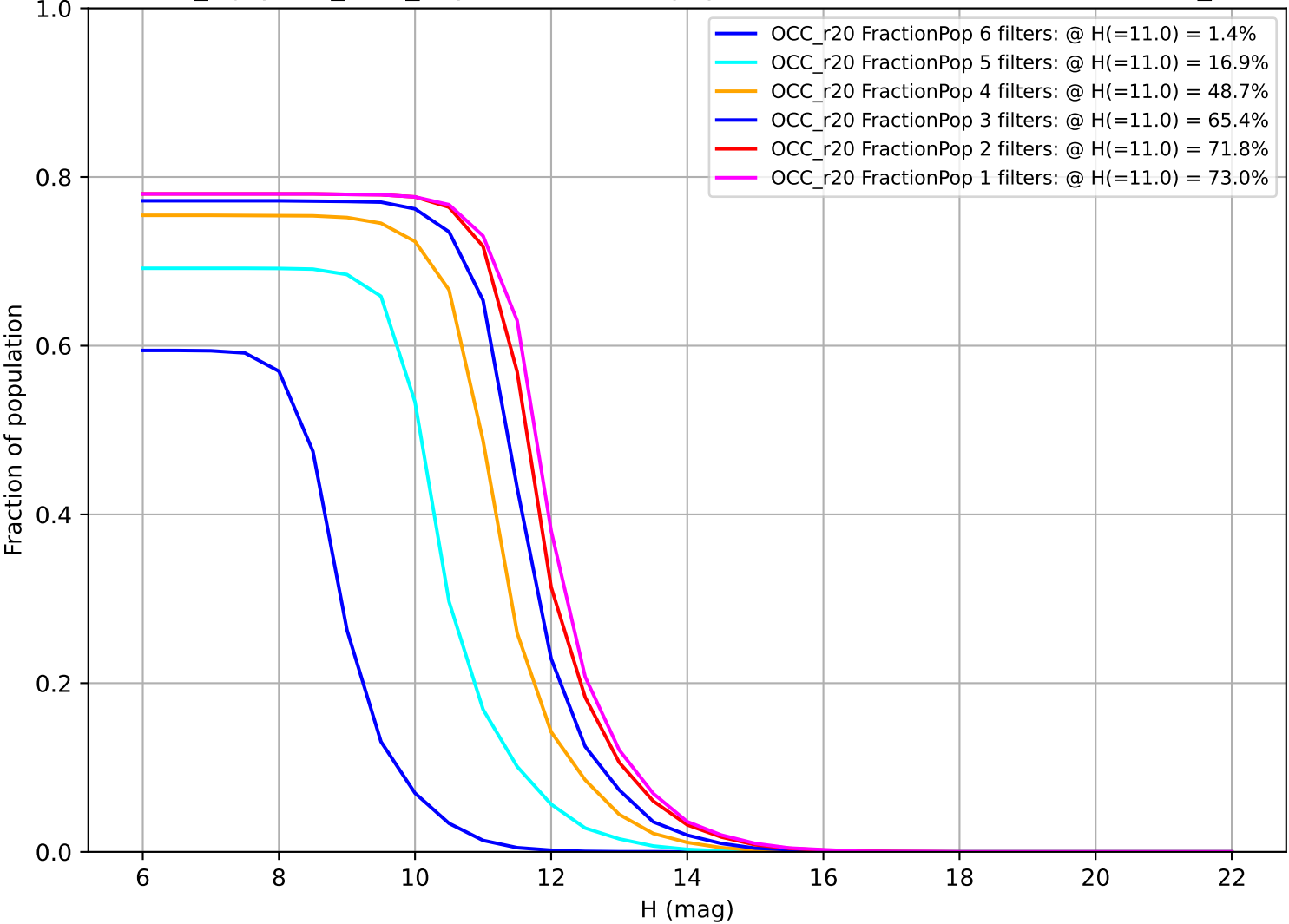
noroll_mjdp180_v3.4_10yrs: Fraction of population with colors in X filters OCC_r20
