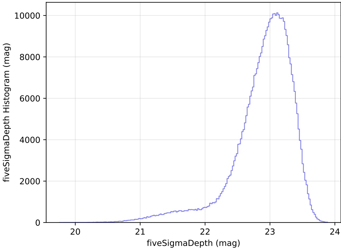
noroll_mjdp180_v3.4_10yrs z: fiveSigmaDepth Histogram
