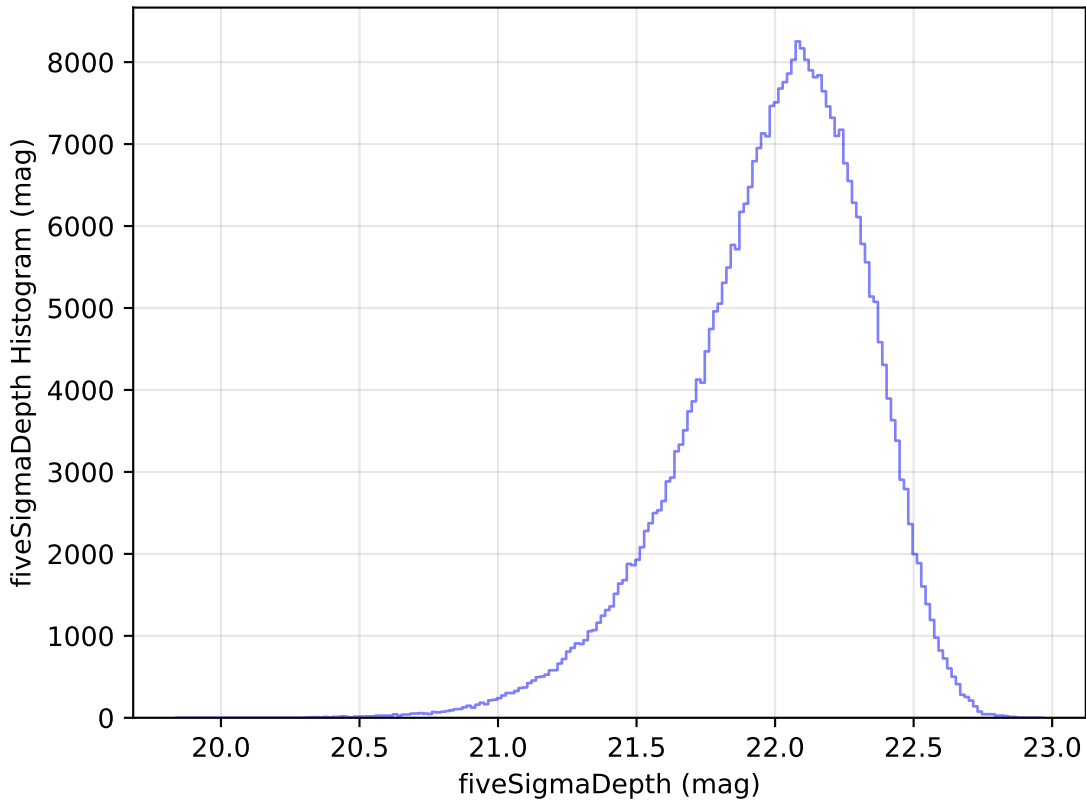
noroll_mjdp180_v3.4_10yrs y: fiveSigmaDepth Histogram
