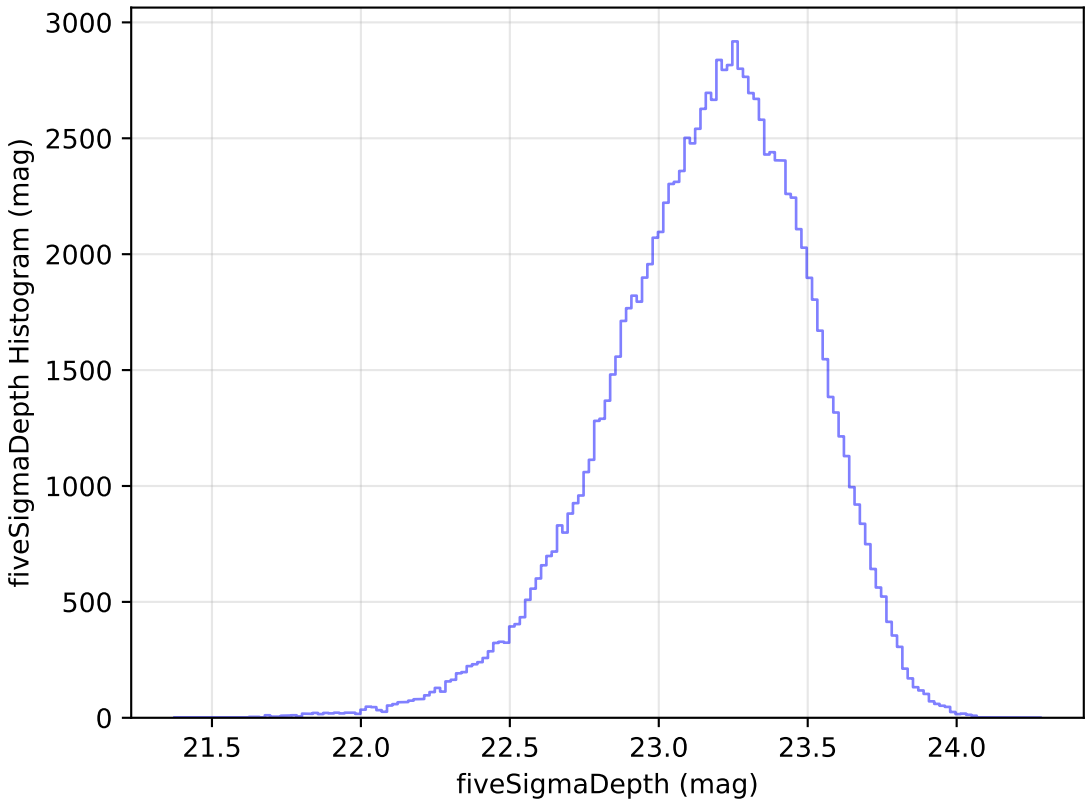
noroll_mjdp180_v3.4_10yrs u: fiveSigmaDepth Histogram
