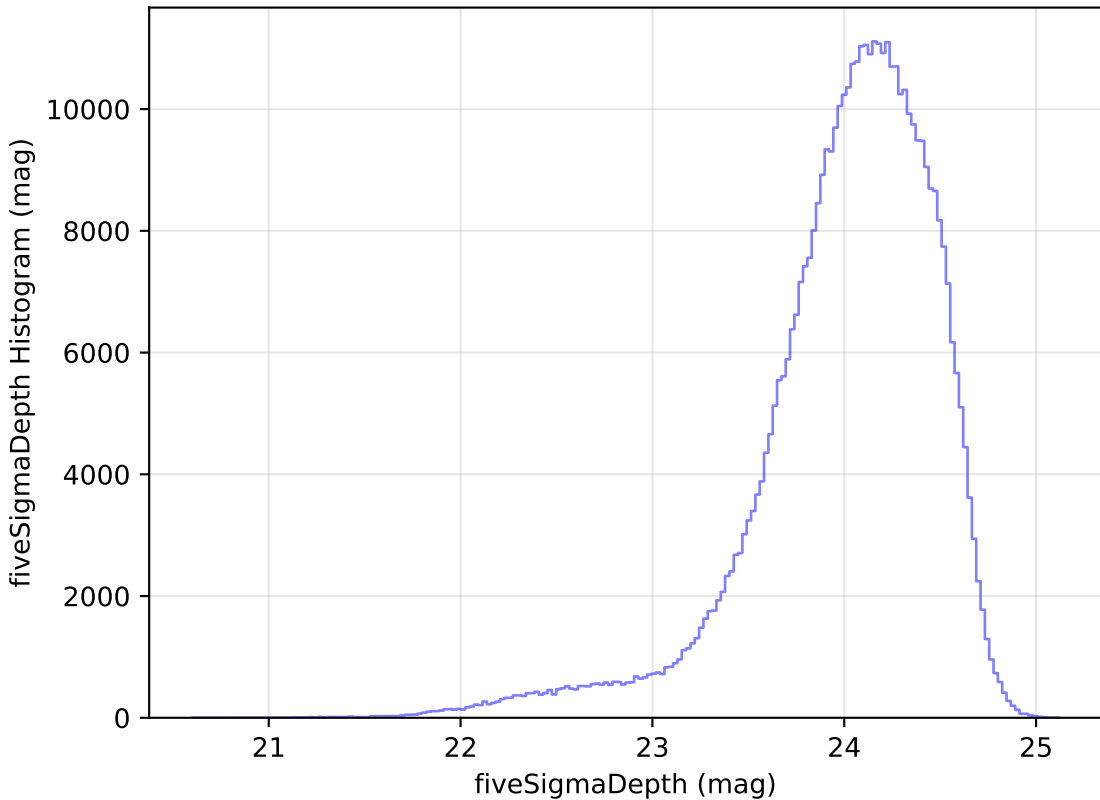
noroll_mjdp180_v3.4_10yrs r: fiveSigmaDepth Histogram
