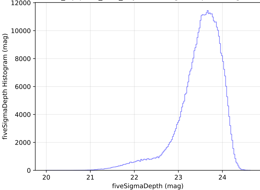
noroll_mjdp180_v3.4_10yrs i: fiveSigmaDepth Histogram
