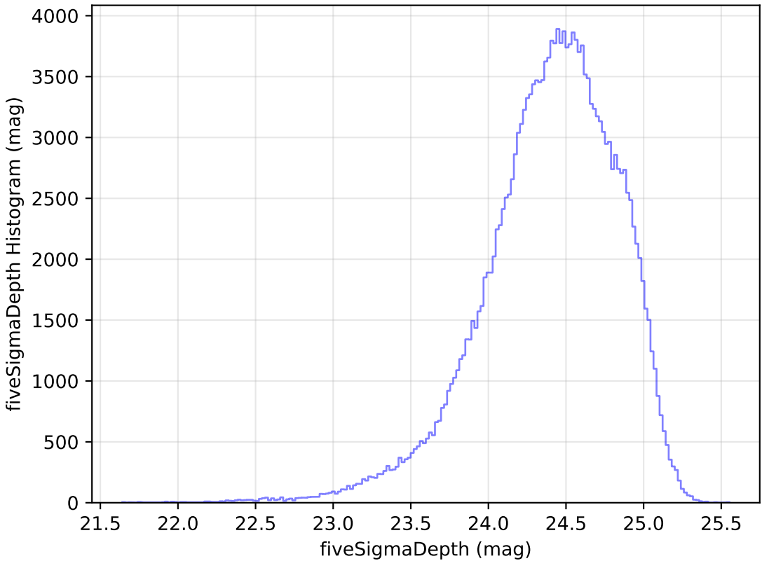
noroll_mjdp180_v3.4_10yrs g: fiveSigmaDepth Histogram
