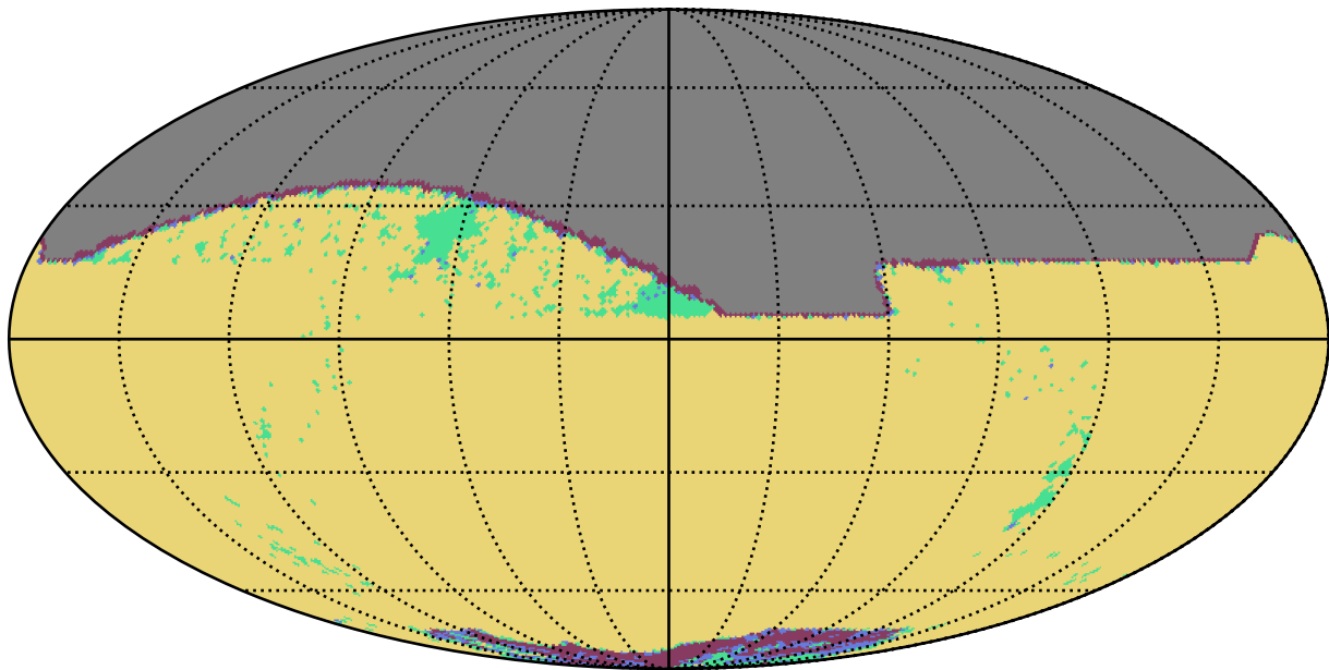
noroll_mjdp180_v3.4_10yrs z band: YearCoverage night
