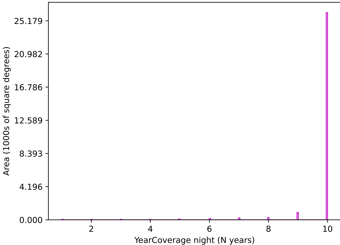
noroll_mjdp180_v3.4_10yrs z band: YearCoverage night
