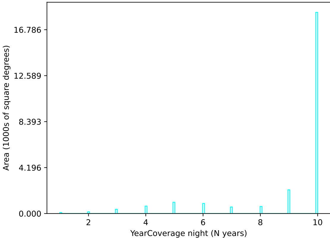
noroll_mjdp180_v3.4_10yrs u band: YearCoverage night
