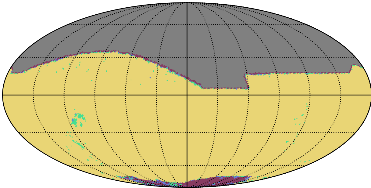
noroll_mjdp180_v3.4_10yrs r band: YearCoverage night
