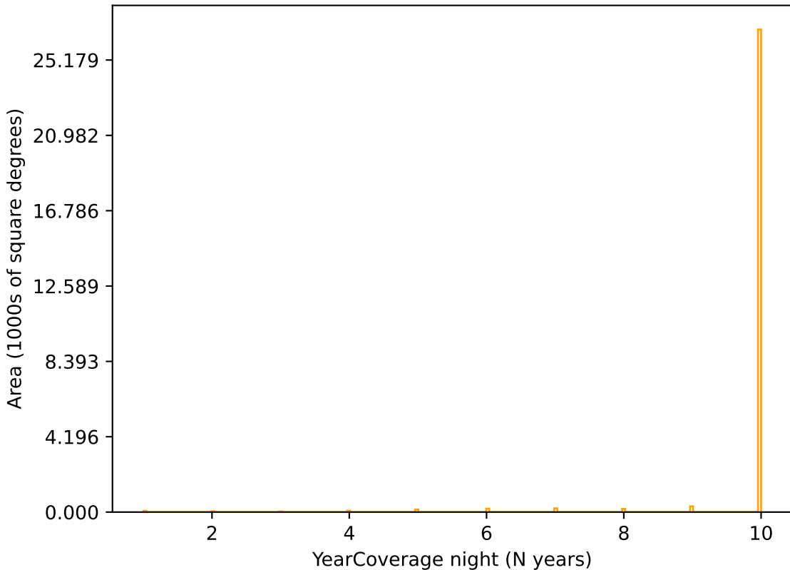
noroll_mjdp180_v3.4_10yrs r band: YearCoverage night
