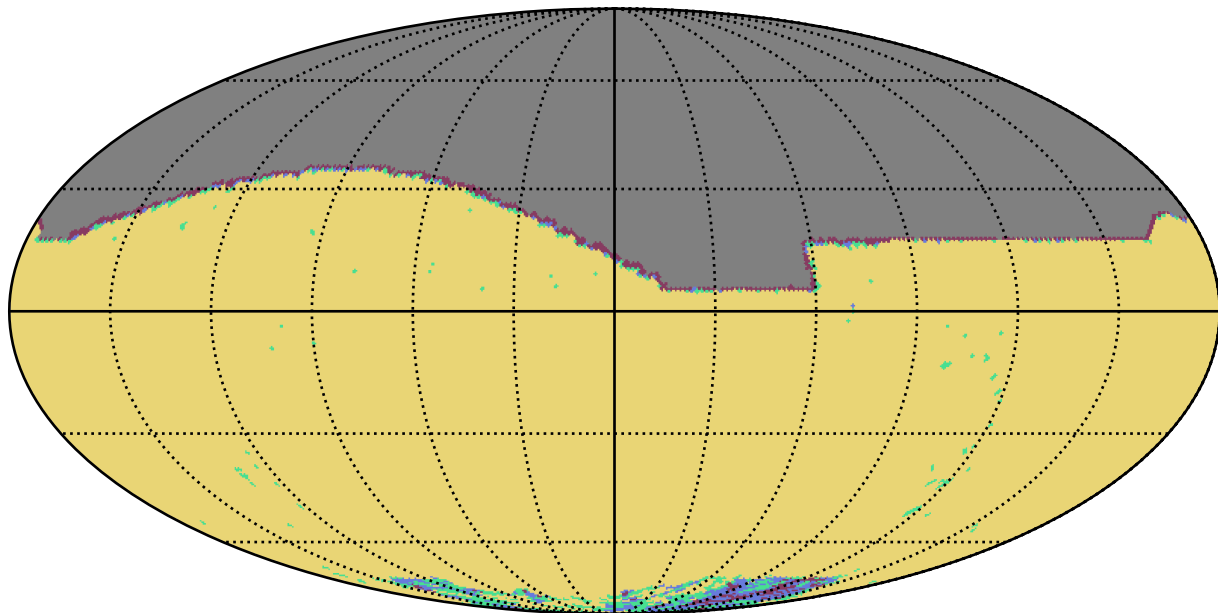
noroll_mjdp180_v3.4_10yrs i band: YearCoverage night
