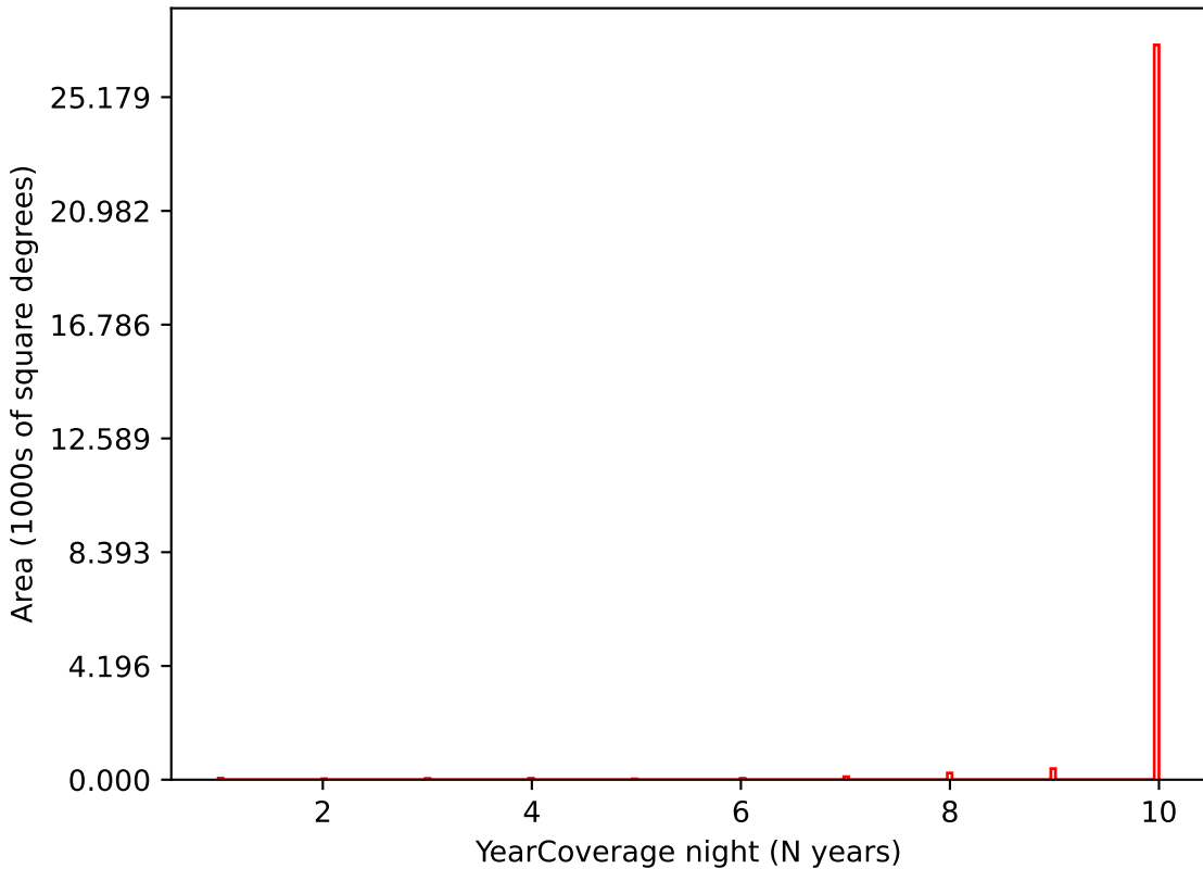
noroll_mjdp180_v3.4_10yrs i band: YearCoverage night
