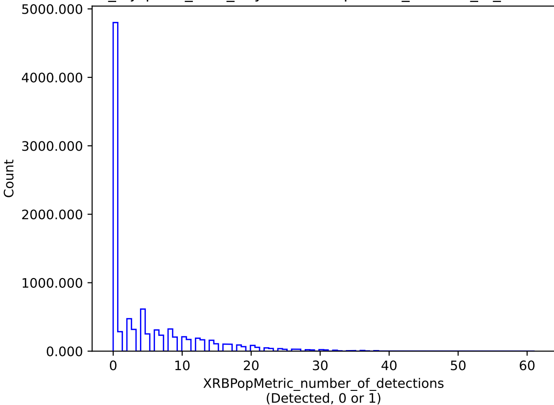
noroll_mjdp180_v3.4_10yrs : XRBPoMetric_number_of_detections
