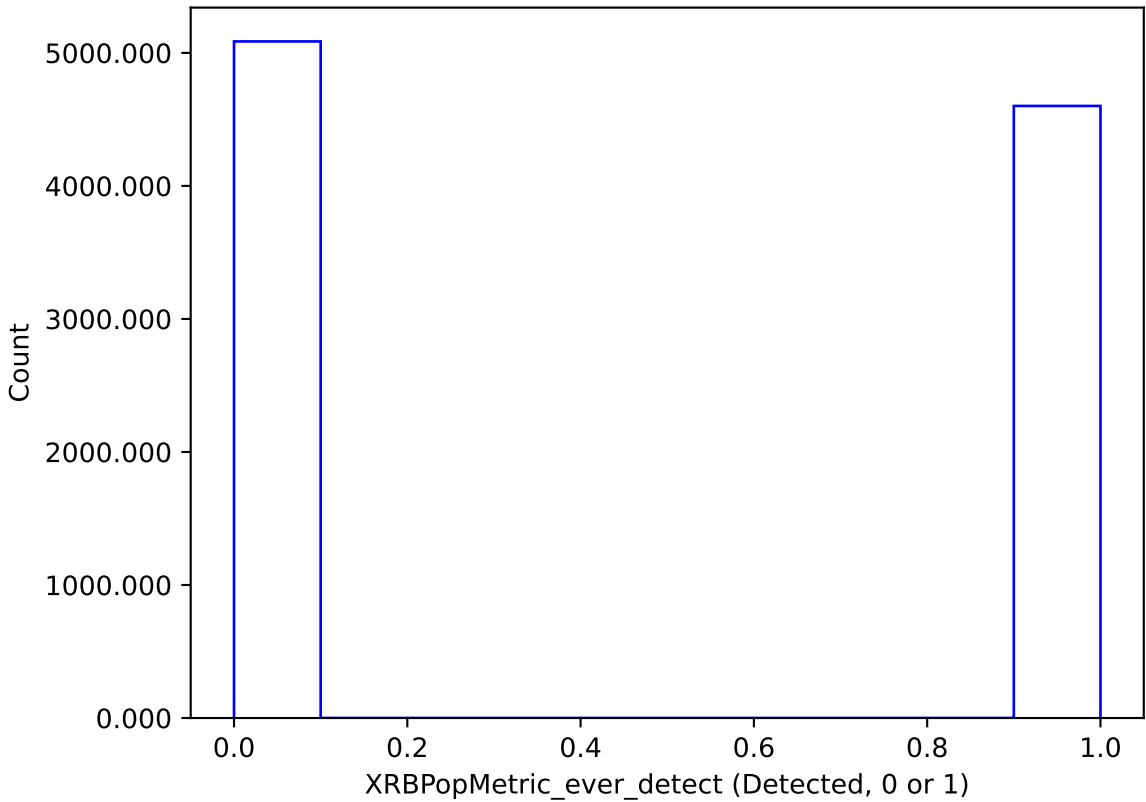
noroll_mjdp180_v3.4_10yrs : XRBPoMetric_ever_detect
