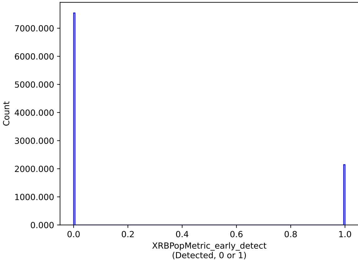
noroll_mjdp180_v3.4_10yrs : XRBPoMetric_early_detect
