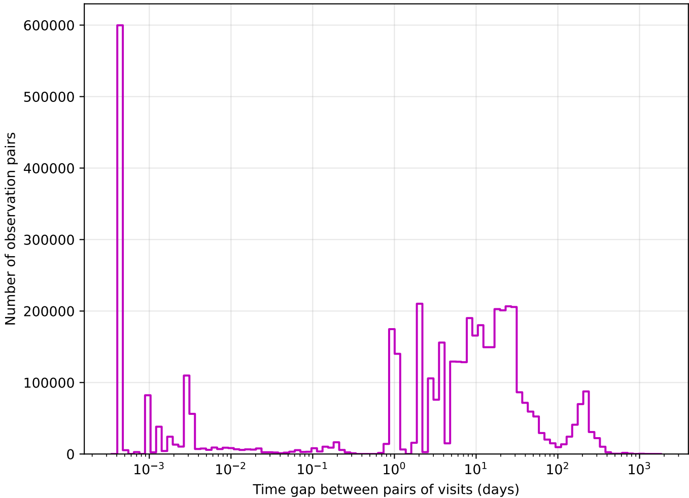
noroll_mjdp180_v3.4_10yrs z band: Tgaps observationStartMJD
