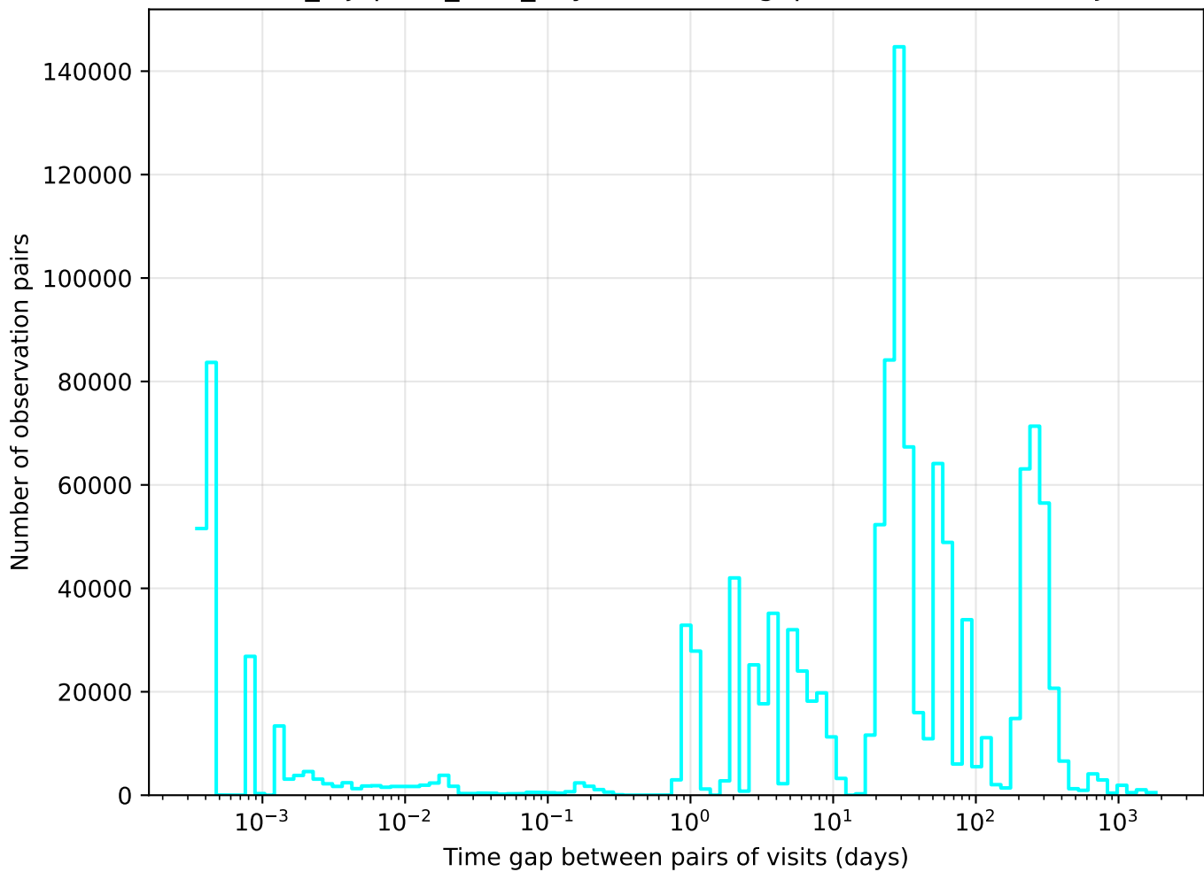
noroll_mjdp180_v3.4_10yrs u band: Tgaps observationStartMJD
