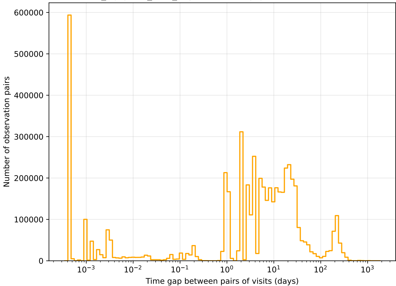
noroll_mjdp180_v3.4_10yrs r band: Tgaps observationStartMJD
