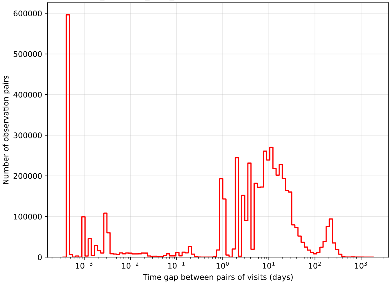
noroll_mjdp180_v3.4_10yrs i band: Tgaps observationStartMJD
