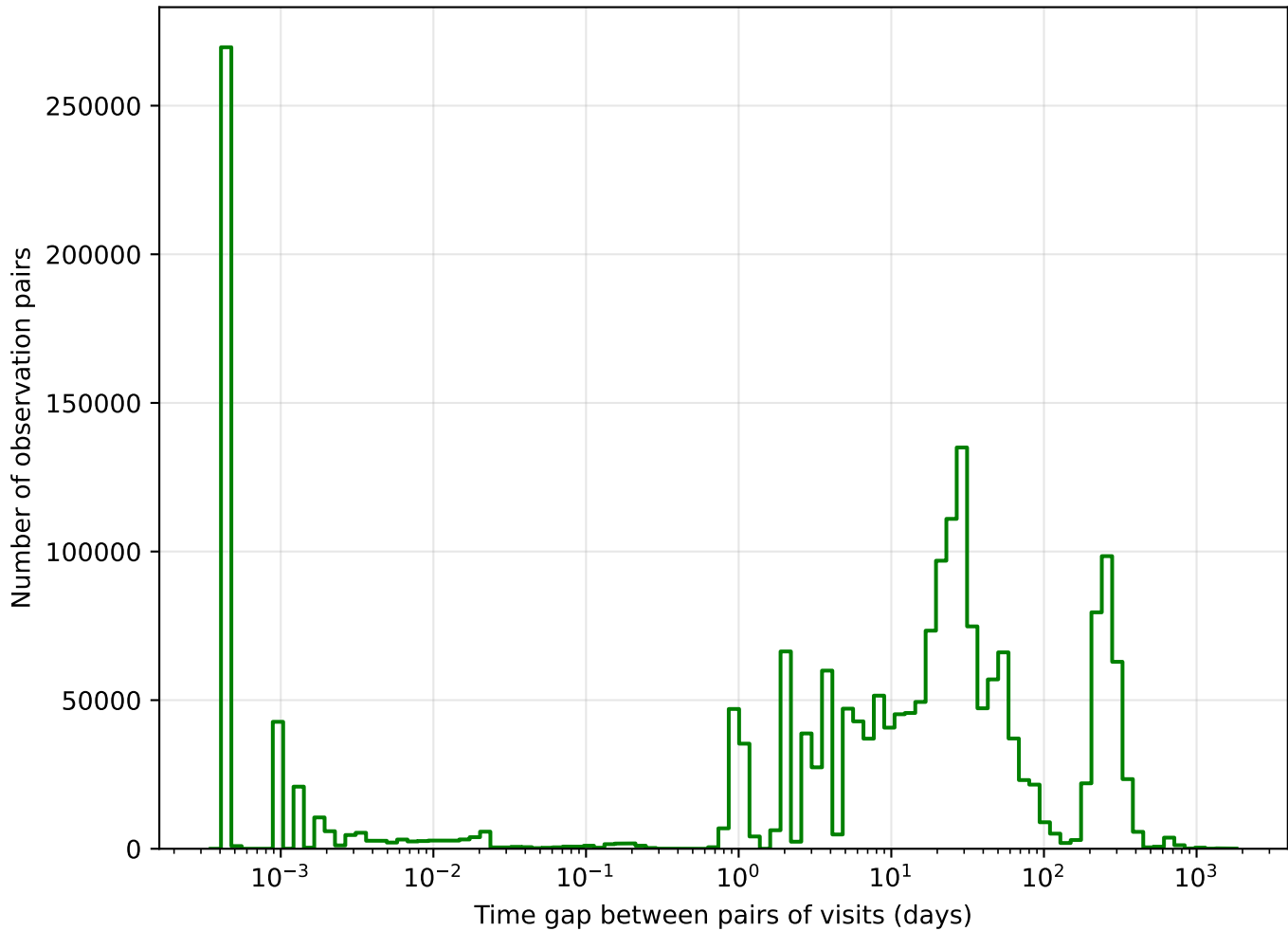
noroll_mjdp180_v3.4_10yrs g band: Tgaps observationStartMJD
