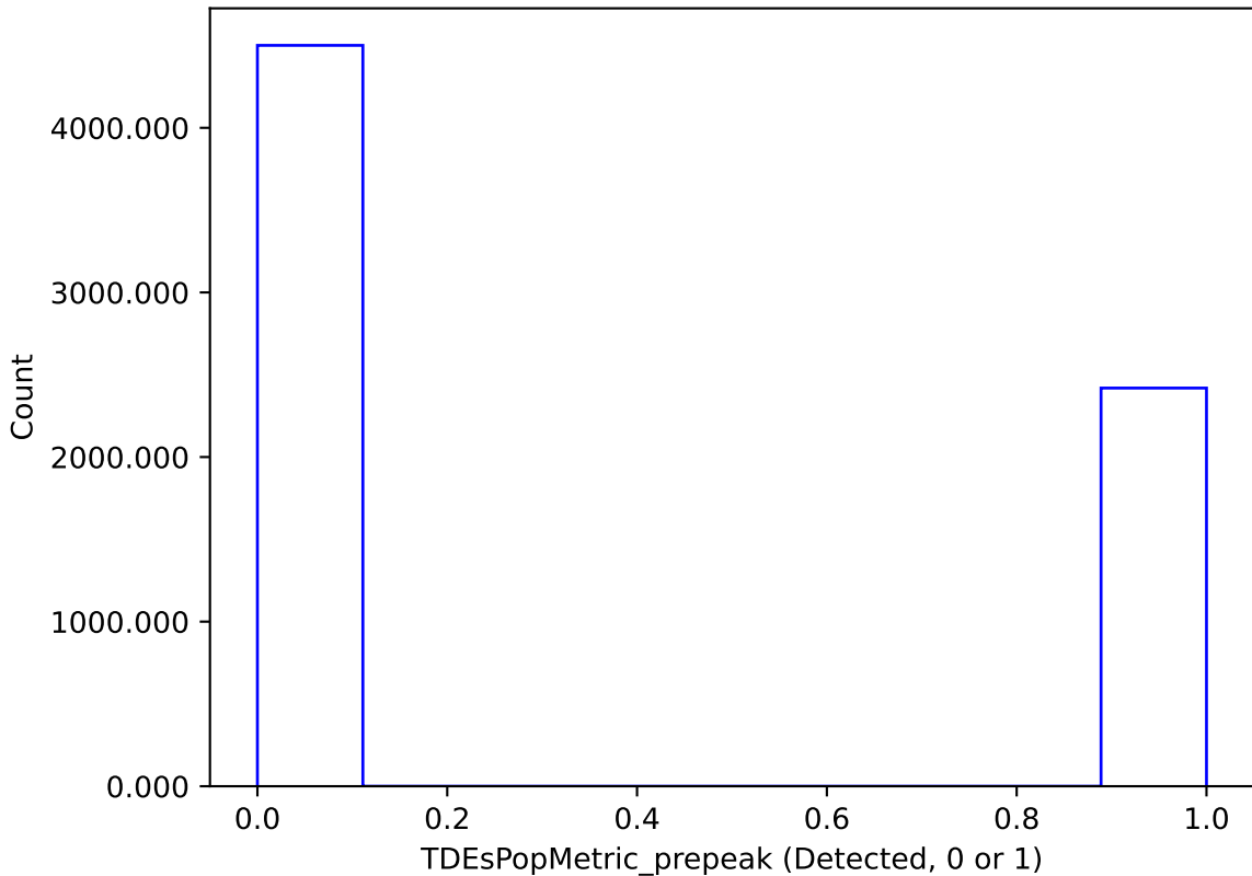
noroll_mjdp180_v3.4_10yrs : TDEsPopMetric_prepeak
