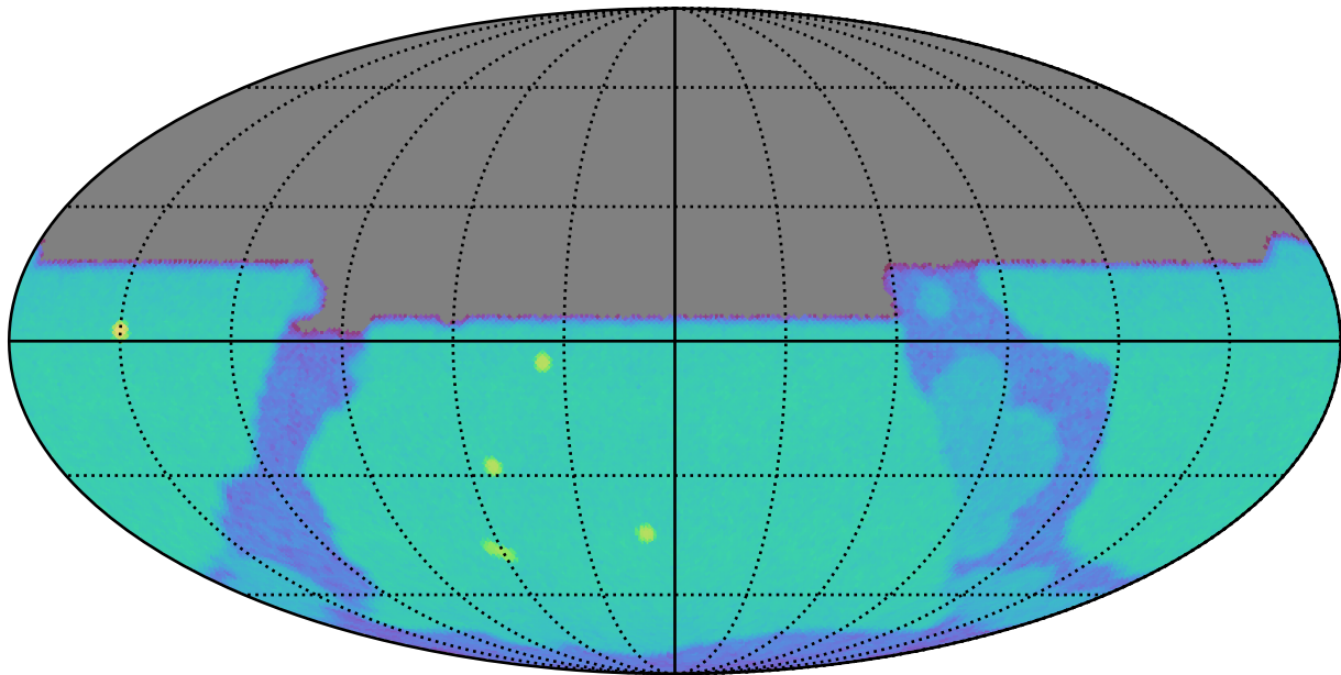
noroll_mjdp180_v3.4_10yrs u: SurfaceBrightLimit
